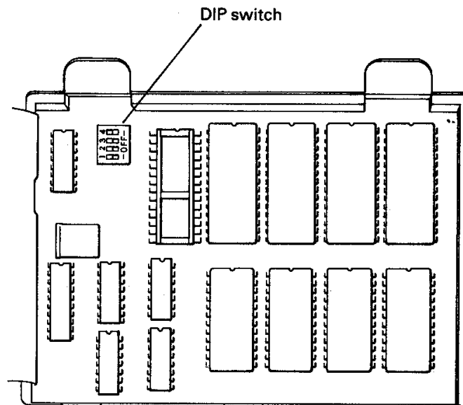
Location of the DIP Switch
